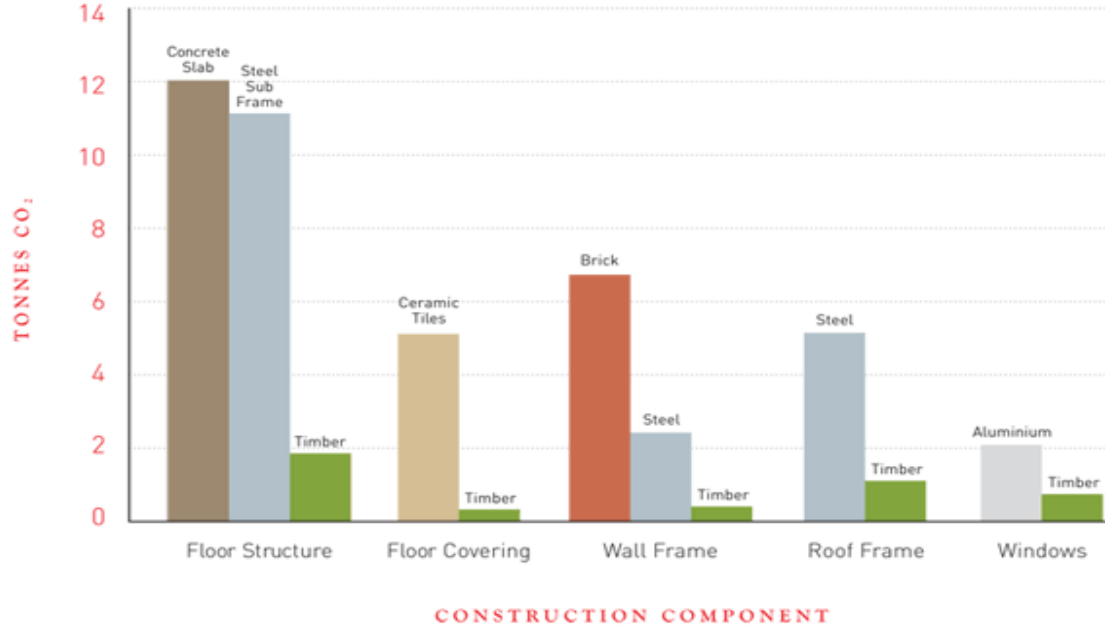
Greenhouse gasses emitted in manufacture of building materials for a single story house
